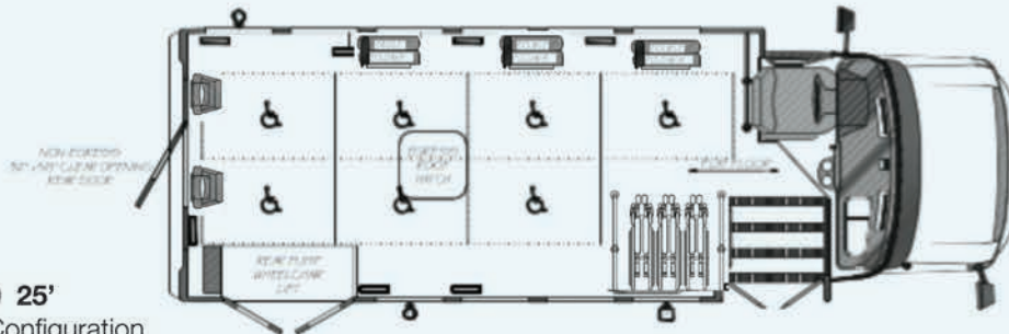
VIP 2200 22' Seating Configuration Driver + 7 ambulatory & 1 wheelchair or driver + 6 wheelchair 9 total capacity, No CDL required
