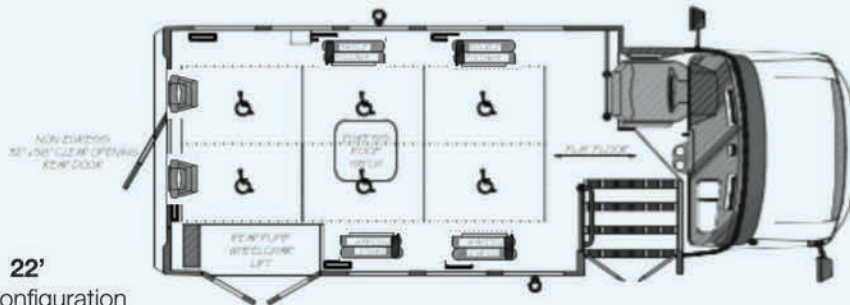
VIP 2500 25' Seating Configuration Driver + 2 Fixed Seats plus 6 wheelchair-ambulatory optional positions 9 total capacity. No CDL required
