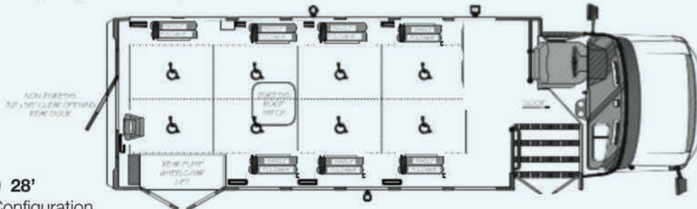
VIP 2500 25' Seating Configuration Driver + 8 ambulatory & 1 wheelchair or driver + 7 wheelchair 9 total max capacity, No CDL required
